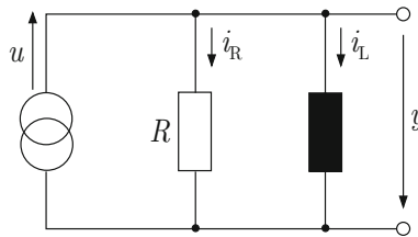
Abb. 4.6: RL-Glied zur Differenziation
