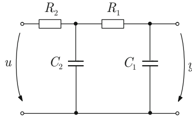
Abb. 4.21: RC-Glied
