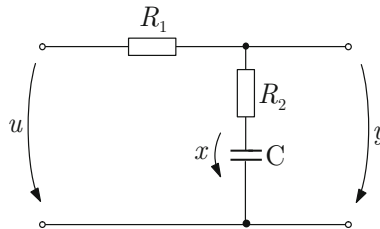
Abb. 5.4: RC-Glied
