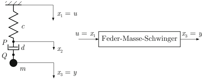
Abb. 4.3: Feder-Masse-Schwinger
