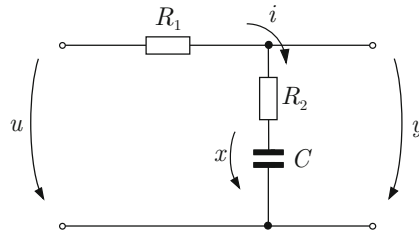
Abb. 6.15: RC-Glied
